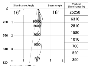
■ Direct Horizontal Illuminance DD140-1015WW9027D
