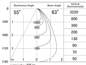
■ Direct Horizontal Illuminance DD140-1050WW9027D
