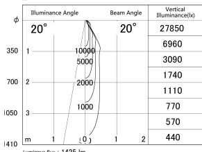
■ Direct Horizontal Illuminance DD140-1520WW9027D
