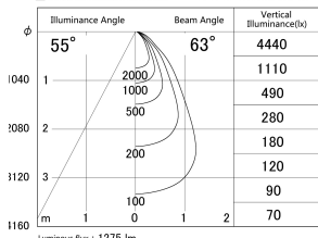
■ Direct Horizontal Illuminance DD140-1550WW9027D
