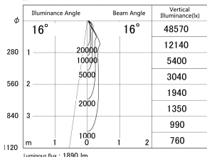
■ Direct Horizontal Illuminance DD140-2015WW9027D
