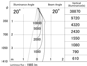
■ Direct Horizontal Illuminance DD140-2020WW9027D
