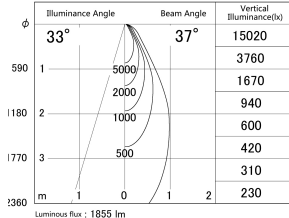
■ Direct Horizontal Illuminance DD140-2030WW9027D
