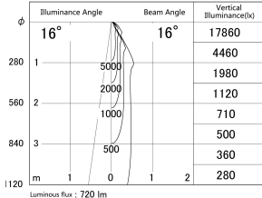
■ Direct Horizontal Illuminance DD140-0815WW9030D
