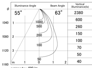
■ Direct Horizontal Illuminance DD140-0850WW9030D
