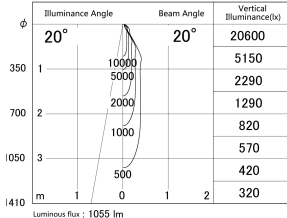
■ Direct Horizontal Illuminance DD140-1020WW9030D
