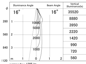
■ Direct Horizontal Illuminance DD140-1515WW9030D
