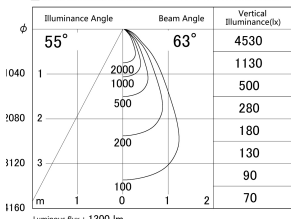
■ Direct Horizontal Illuminance DD140-1550WW9030D
