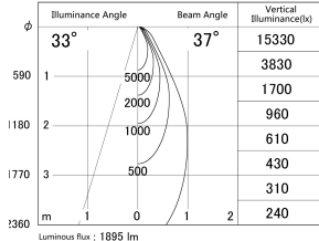
■ Direct Horizontal Illuminance DD140-2030WW9030D
