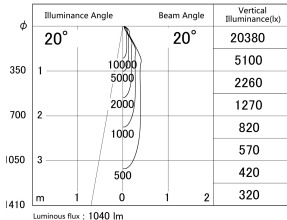
■ Direct Horizontal Illuminance DD140-1020WW9035D
