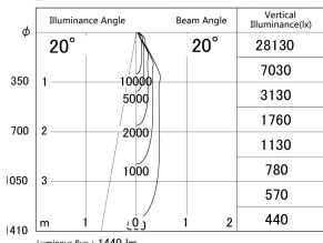
■ Direct Horizontal Illuminance DD140-1520WW9035D
