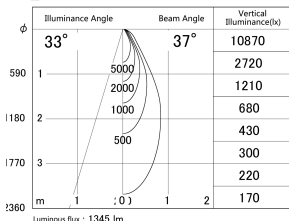
■ Direct Horizontal Illuminance DD140-1530WW9035D
