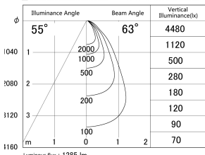
■ Direct Horizontal Illuminance DD140-1550WW9035D
