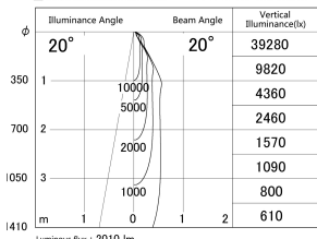
■ Direct Horizontal Illuminance DD140-2020WW9035D
