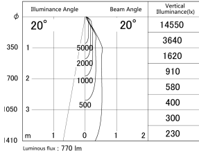
■ Direct Horizontal Illuminance DD140-0820WW9040D
