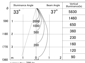
■ Direct Horizontal Illuminance DD140-0830WW9040D
