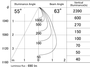
■ Direct Horizontal Illuminance DD140-0850WW9040D
