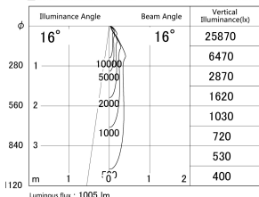
■ Direct Horizontal Illuminance DD140-1015WW9040D
