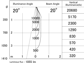
■ Direct Horizontal Illuminance DD140-1020WW9040D
