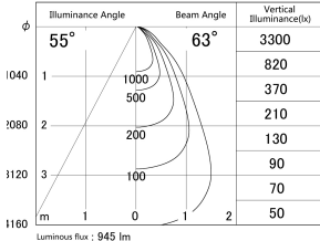
■ Direct Horizontal Illuminance DD140-1050WW9040D
