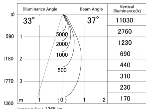
■ Direct Horizontal Illuminance DD140-1530WW9040D
