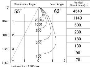
■ Direct Horizontal Illuminance DD140-1550WW9040D
