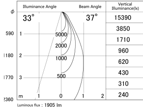
■ Direct Horizontal Illuminance DD140-2030WW9040D
