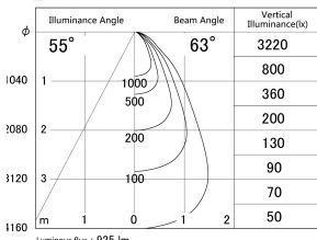
Direct Horizontal Illuminance DD140-1050WB9027D
