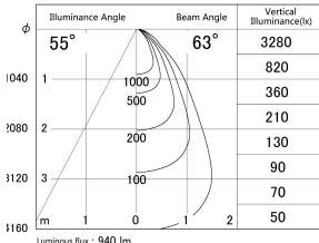
■ Direct Horizontal Illuminance DD140-1050WB9030D
