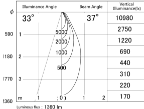
■ Direct Horizontal Illuminance DD140-1530WB9030D
