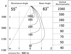
■ Direct Horizontal Illuminance DD140-0850WB9035D
