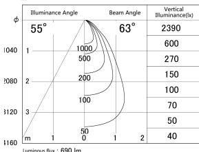
Direct Horizontal Illuminance DD140-0850WB9040D
