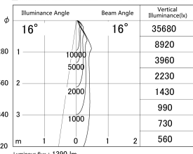
Direct Horizontal Illuminance DD140-1515WB9040D
