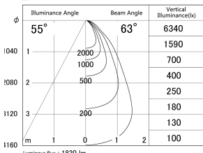
■ Direct Horizontal Illuminance DD140-2050WB9040D
