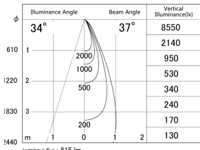
■ Direct Horizontal Illuminance DD155-0835MW9027
