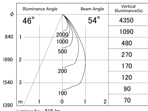
■ Direct Horizontal Illuminance DD155-0855MW9027
