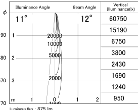
■ Direct Horizontal Illuminance DD155-1010MW9027
