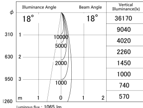
■ Direct Horizontal Illuminance DD155-1015MW9027
