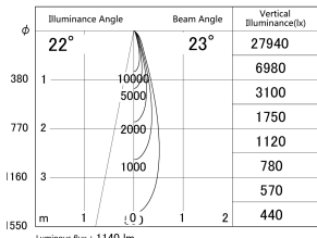
■ Direct Horizontal Illuminance DD155-1025MW9027
