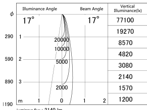
■ Direct Horizontal Illuminance DD155-2015MW9027
