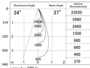
■ Direct Horizontal Illuminance DD155-2035MW9027
