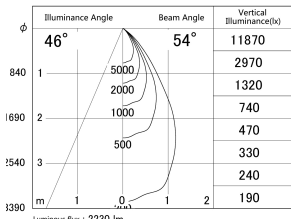
■ Direct Horizontal Illuminance DD155-2055MW9027
