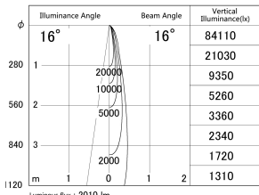
■ Direct Horizontal Illuminance DD155-2515MW9027
