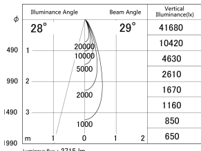
■ Direct Horizontal Illuminance DD155-2530MW9027
