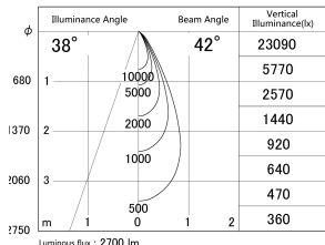
■ Direct Horizontal Illuminance DD155-2540MW9027
