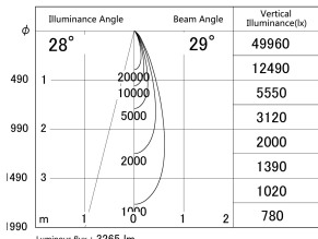
■ Direct Horizontal Illuminance DD155-3030MW9027
