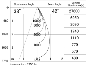
■ Direct Horizontal Illuminance DD155-3040MW9027
