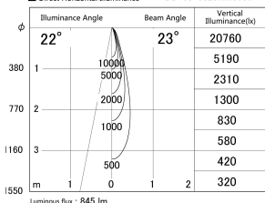
■ Direct Horizontal Illuminance DD155-0825MW9030
