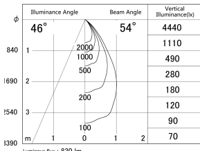
■ Direct Horizontal Illuminance DD155-0855MW9030
