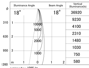
■ Direct Horizontal Illuminance DD155-1015MW9030
